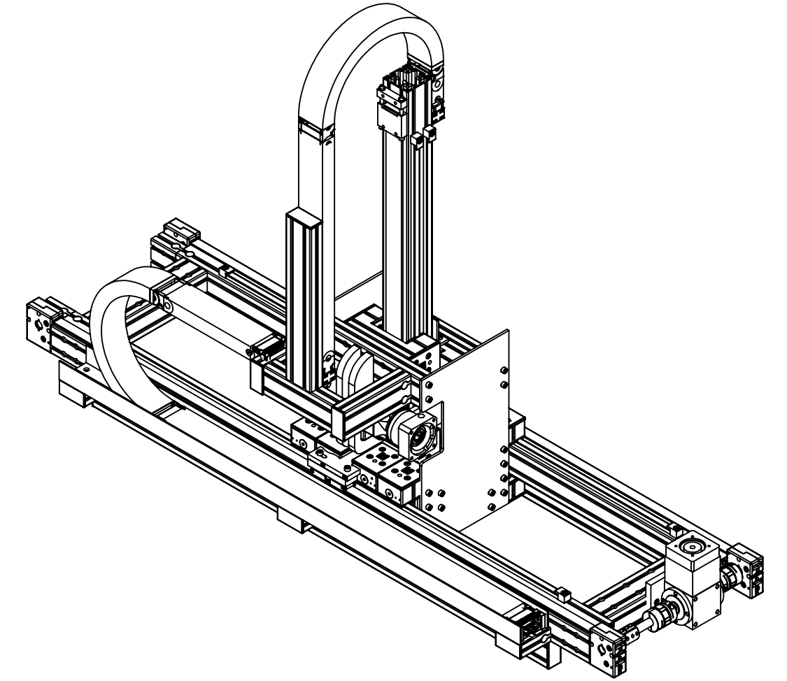
*VCT-090 GEARBOX AND MPG-084 GEARBOX SHOWN IN THIS SYSTEM
